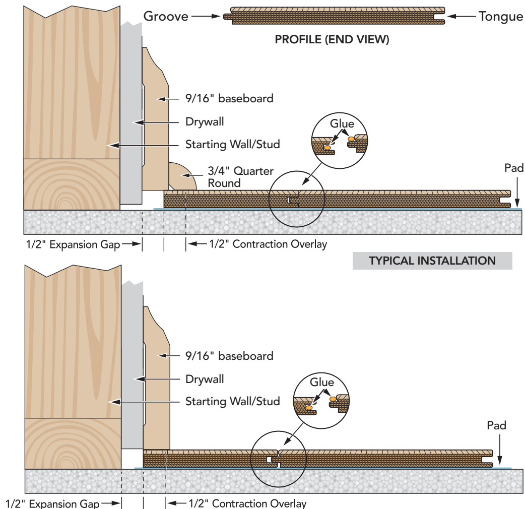
How to achieve required Expansion Gap / Contraction Overlay using base board only
