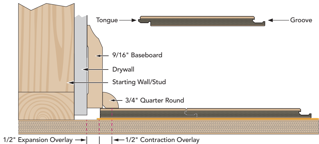
TYPICAL INSTALLATION
