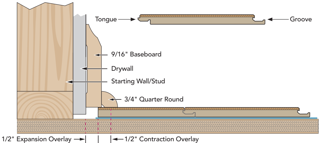
TYPICAL INSTALLATION
