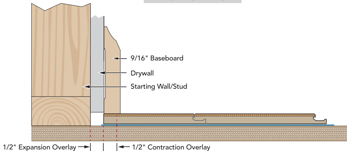
How to achieve required Expansion Gap / Contraction Overlay using base board only
