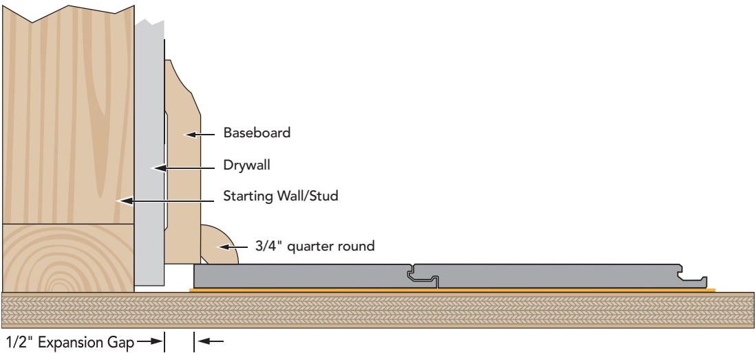
TYPICAL INSTALLATION
