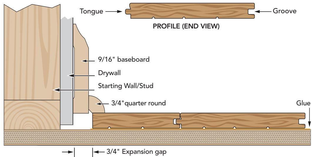
TYPICAL INSTALLATION
