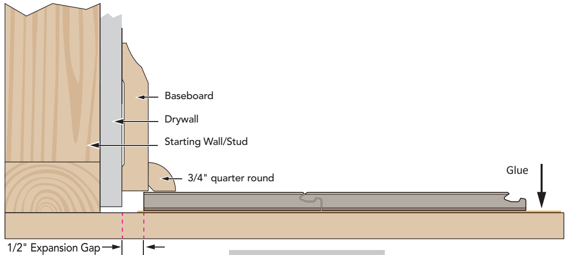
TYPICAL INSTALLATION
