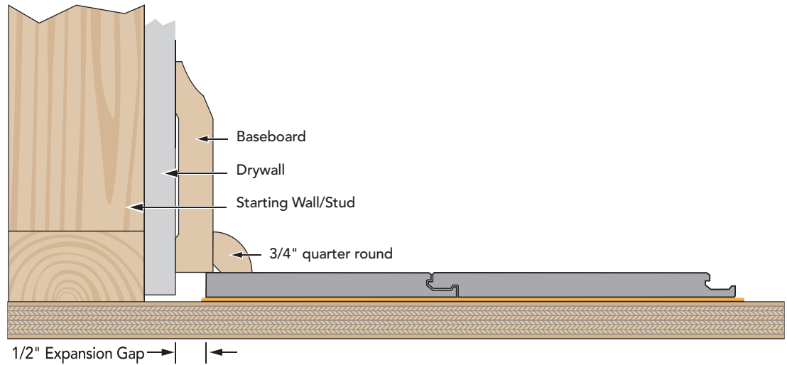
TYPICAL INSTALLATION
