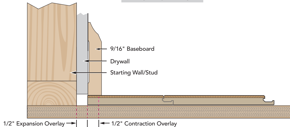
How to achieve required Expansion Gap / Contraction Overlay using base board only
