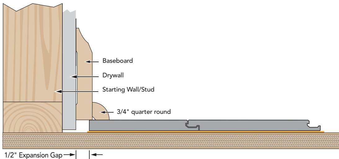
TYPICAL INSTALLATION
