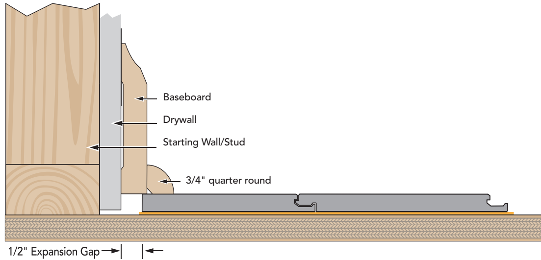
TYPICAL INSTALLATION
