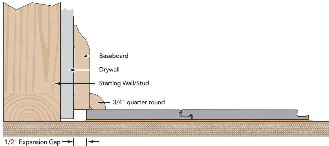
TYPICAL INSTALLATION
