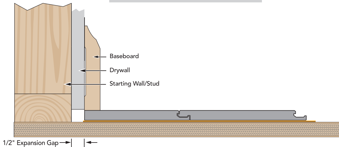
How to achieve required Expansion Gap using base board only
